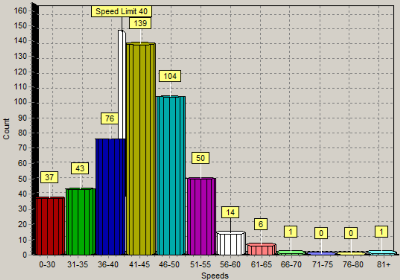
Count vs. Speed 6/20/2019 08:00 am - 6/20/2019 04:00 pm
