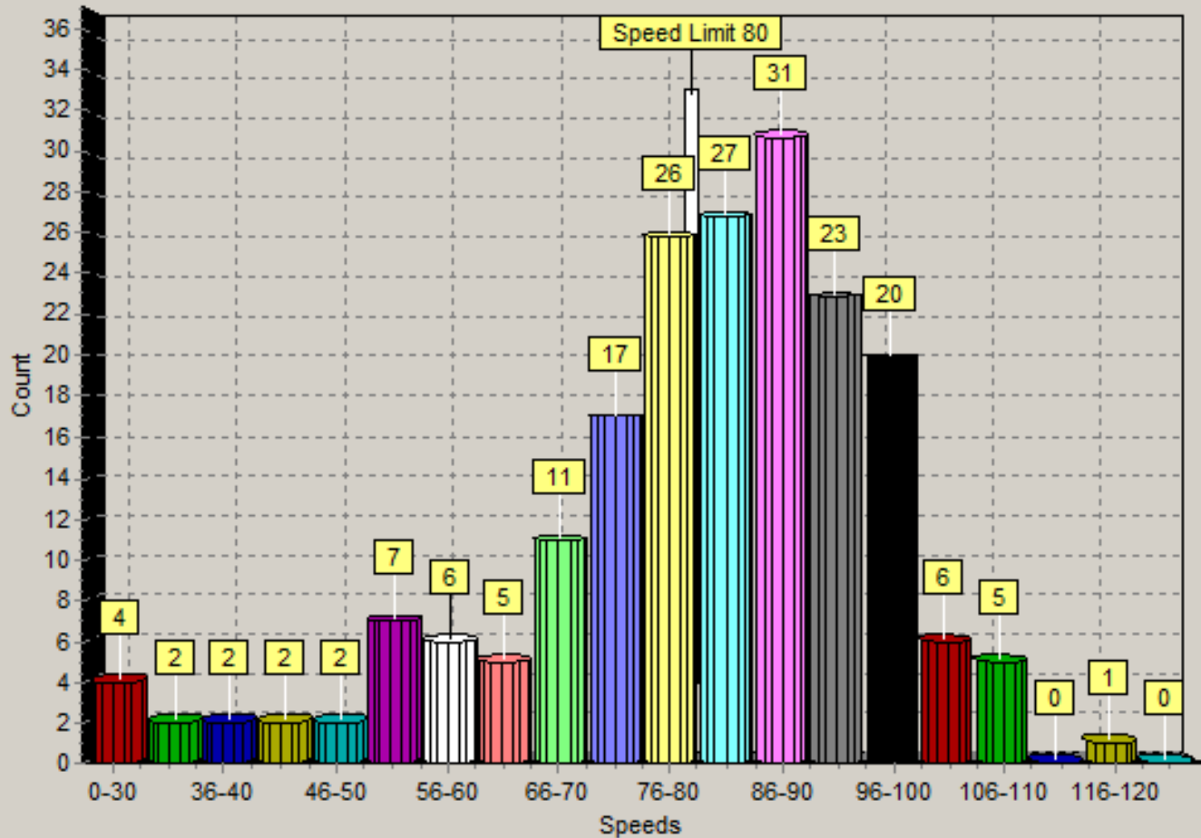
Count vs. Speed 8/19/2019 07:00 am - 8/19/2019 05:00 pm
