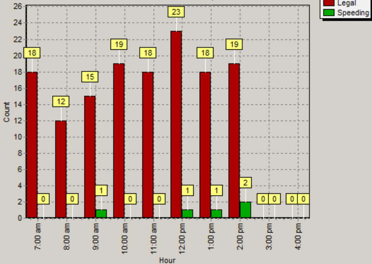
Count vs. Hour 8/7/2019 07:00 am - 8/7/2019 05:00 pm
