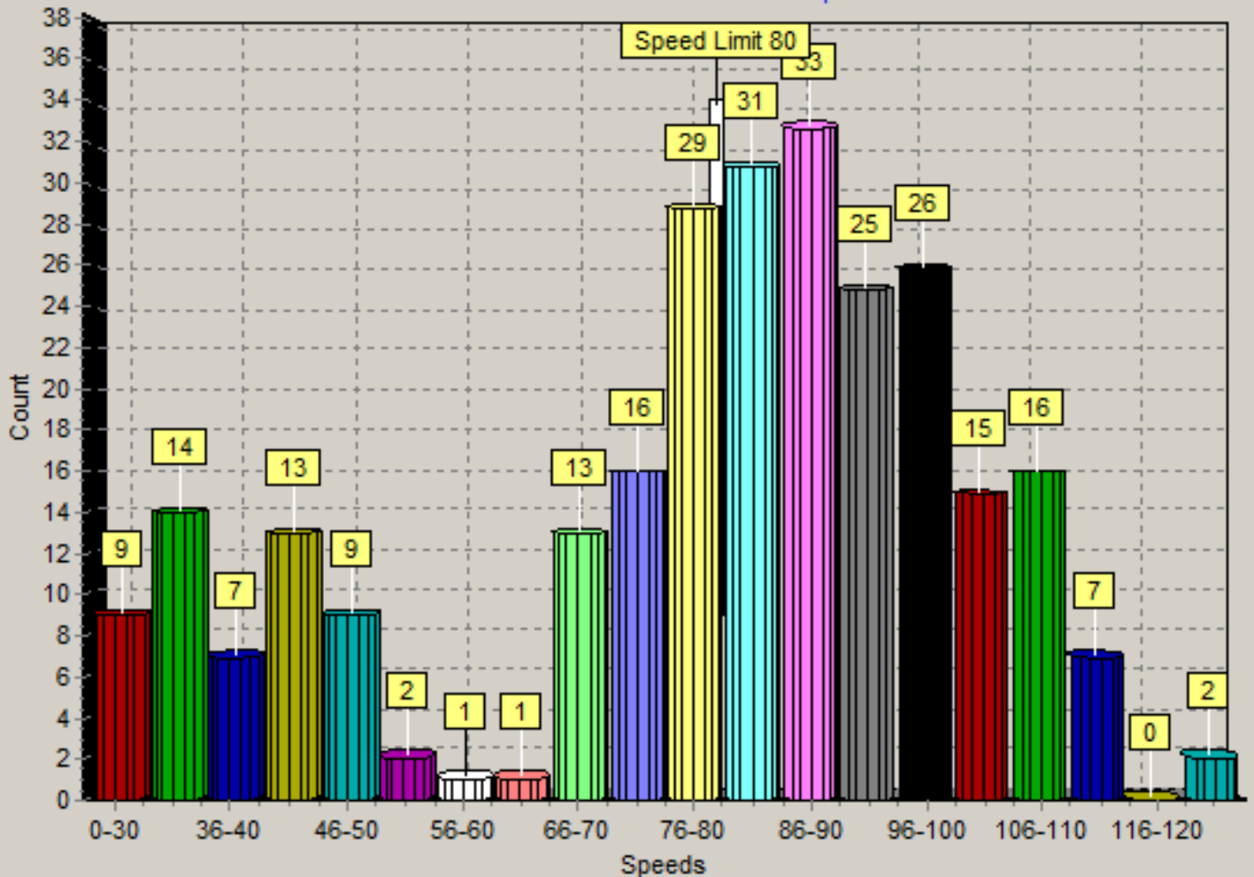
Count vs. Speed 8/20/2019 07:00 am - 8/20/2019 05:00 pm
