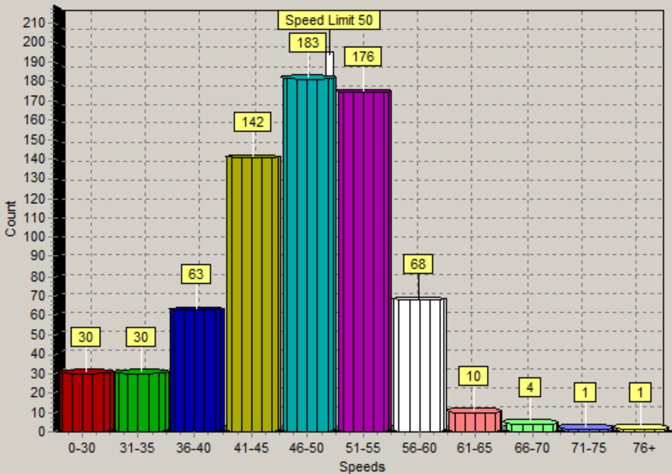
Count vs. Speed 6/26/2019 07:00 am - 6/26/2019 09:00 pm
