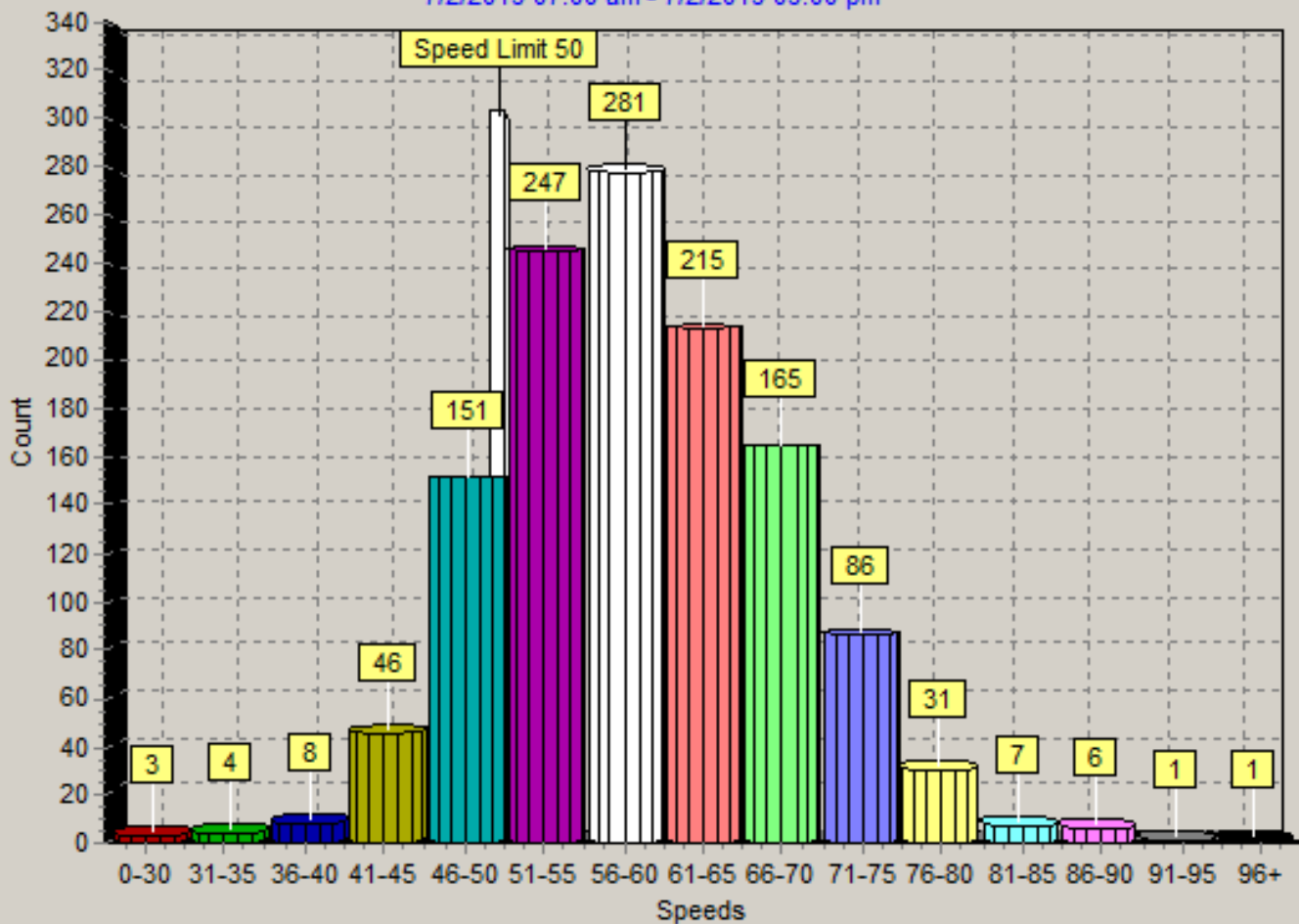
Count vs. Speed 7/2/2019 07:00 am - 7/2/2019 09:00 pm
