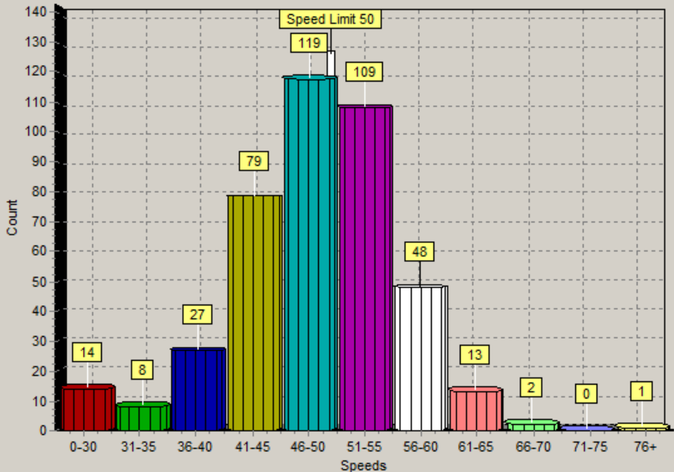
Count vs. Speed 6/25/2019 07:00 am - 6/25/2019 05:00 pm
